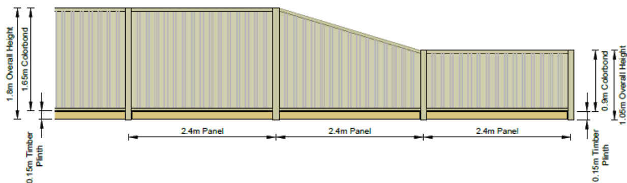
Fencing template for side boundary fencing on all lots in Stage 3
